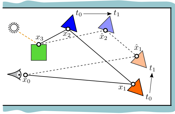
Figure 10: Path warping: an initial path is sampled and evaluated at t = t_0 . The shifted technique yields the path \bar{\mathbf{x}}(t_1) = (\mathbf{x}_0, \hat{\mathbf{x}}_1, \hat{\mathbf{x}}_2, \dots) at t = t_1 .
