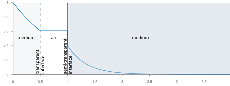
Figure 1: Transmittance across different volumes bounded by fully transparent and semi-transparent interfaces. Free-path sampling typically aims to sample proportional to that profile, which involves alternatingly sampling within the media and potentially transparent surface boundaries until termination.
